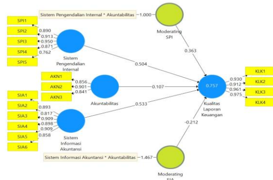
Gambar 2. Hasil Analisis Algorithm Loading Factor
